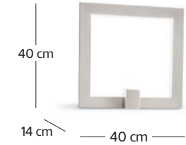
art. Ri_quadro LG LED 2250 LM 20 W 3000 K
