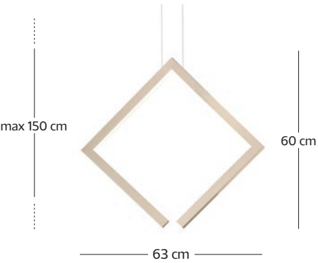
art. Ri_quadro S1 LED 2500 LM 21 W 3000 K
