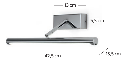
art. Stiled A 42 LED 7,5 W 3000 K 400 lm - Driver incluso / Driver included
